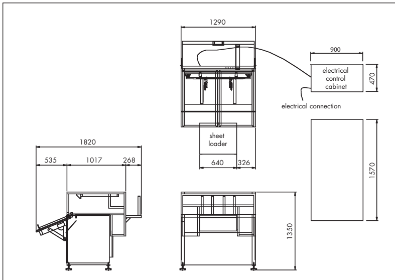
OSG800 SINGLE GUILLOTINE FOOTPRINT
