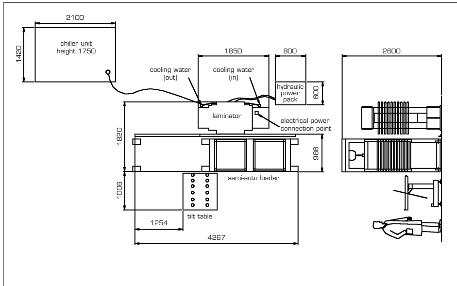
OSS2-10 SINGLE STACK LAMINATOR FOOTPRINT
