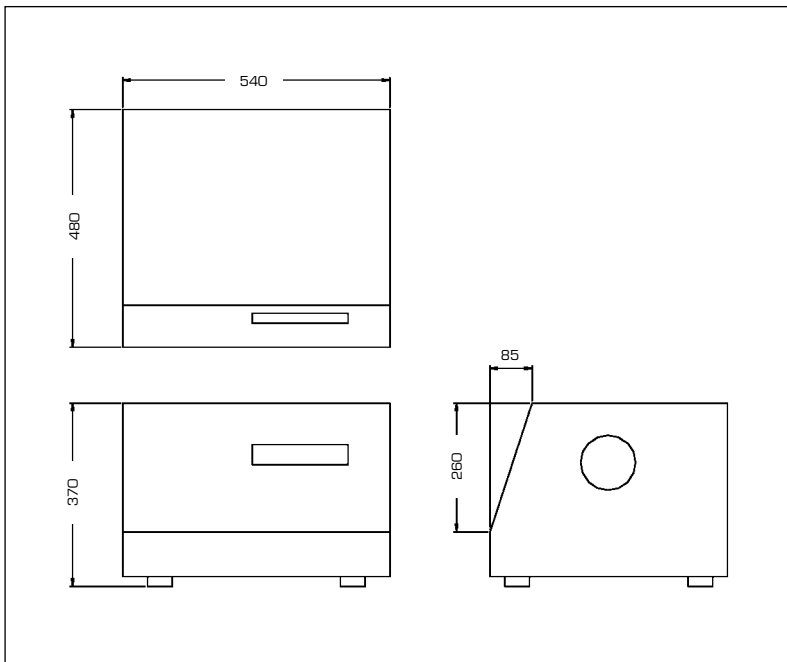
OLA6 LAMINATOR FOOTPRINT
