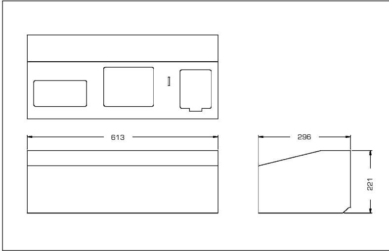
OFT100 FLEX TESTER FOOTPRINT
