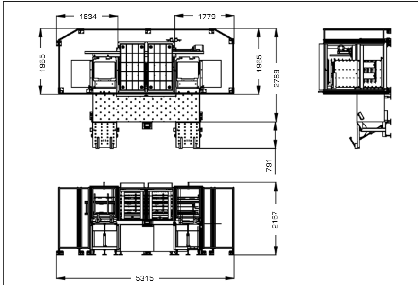
FOOTPRINT DRAWING FOR OMTS1-4 WITH OPTIONAL TILT TABLE
