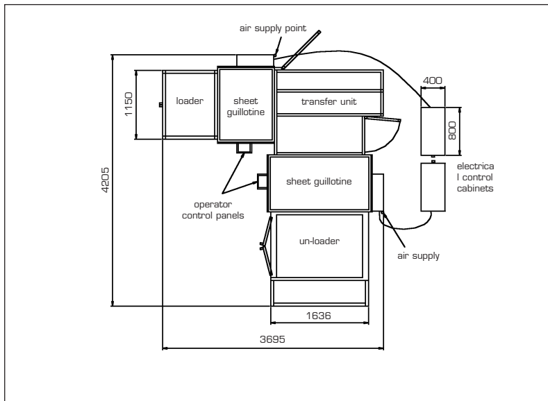
ODG600 DOUBLE GUILLOTINE FOOTPRINT
