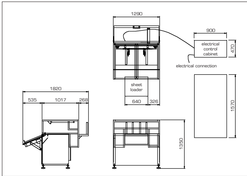
OSG800 SINGLE GUILLOTINE FOOTPRINT
