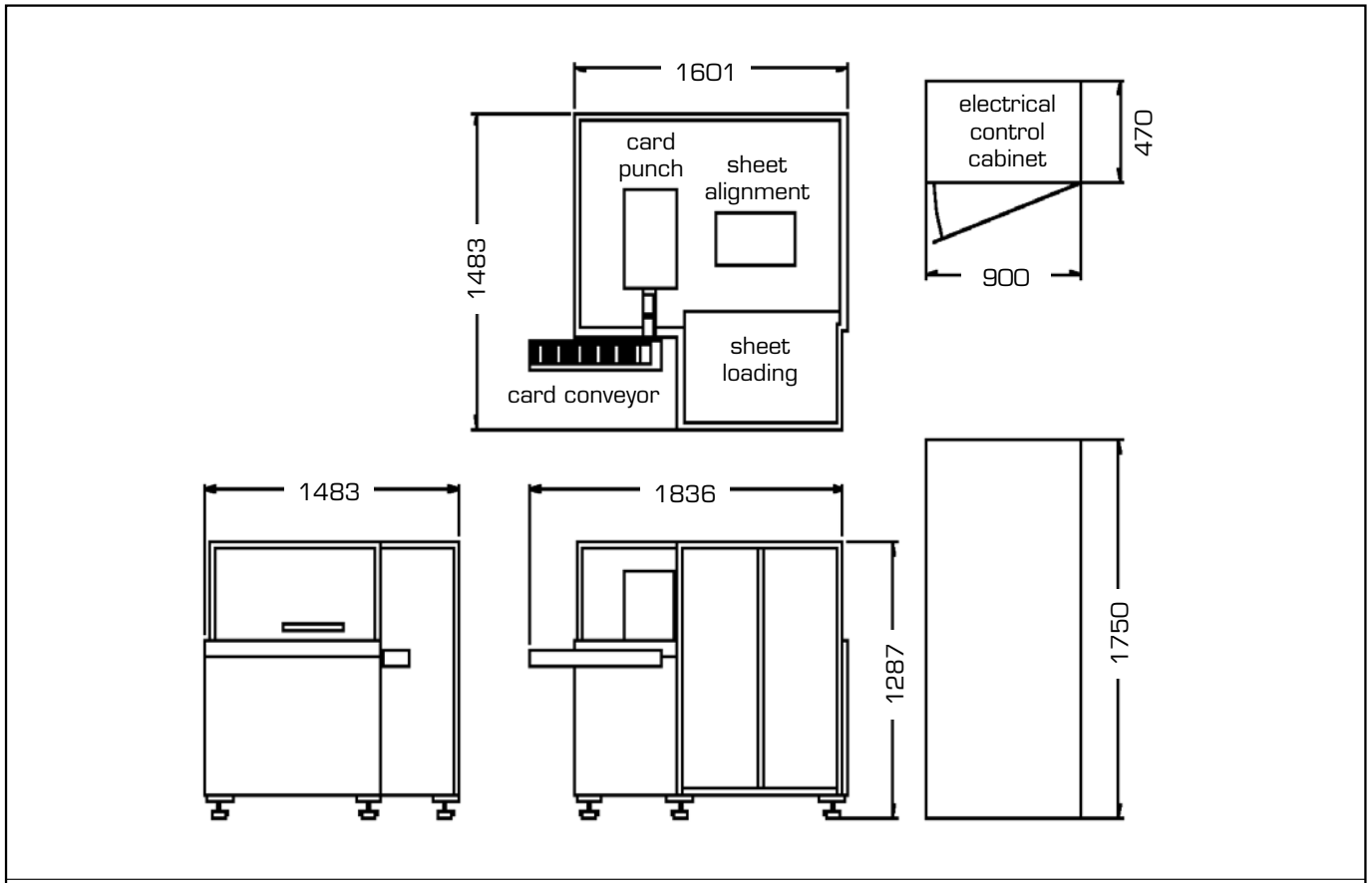
OCP 313A AUTOMATIC SHEET FEED WITH SHINGLING CARD EXIT CONVEYOR
