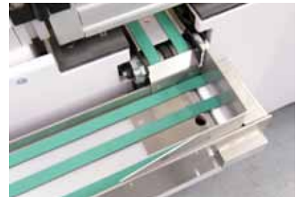
Shingling Exit conveyor
