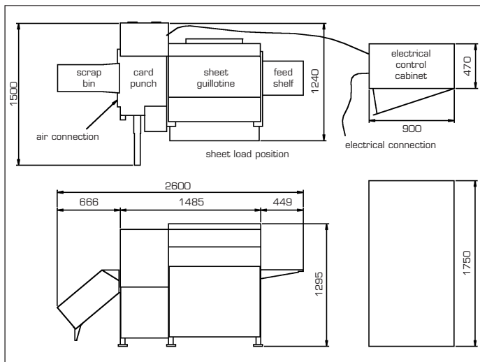
OCP201 MANUAL PUNCH FOOTPRINT
