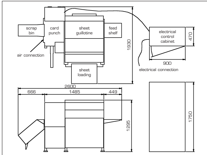
OCP201A AUTO PUNCH FOOTPRINT
